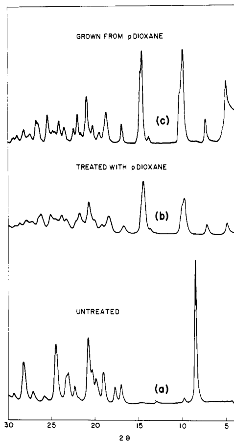
Figure 1. Powder X-ray diffraction patterns (Cu K\alpha radiation) of the orange phase (a), the blue phase obtained by exposing the orange phase to p -dioxane vapor (b), and the blue phase obtained by crystallizing HD_mTU from p -dioxane/water (c).
