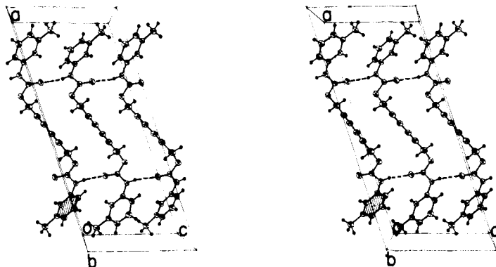
Figure 4. A view of the packing of molecules of HD 10 TU in crystals of the orange phase. The phenyl ring in the reference half-molecule is shaded. The molecules related by the C centering are not shown.
